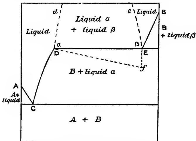
FIG. 37.—Partial miscibility.
